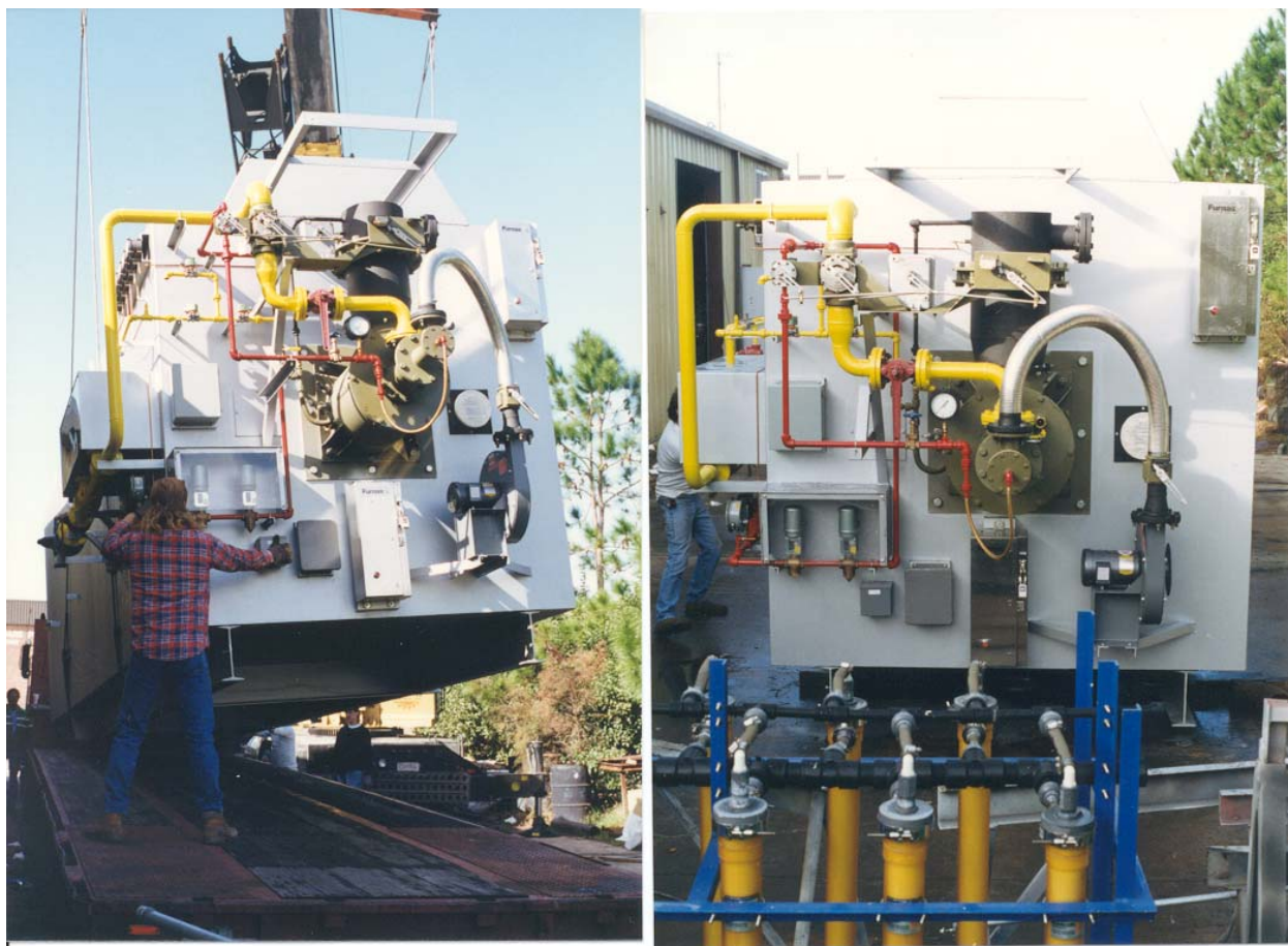
Process waste gas incinerator for Imperial Chemical Industries, Joslin, Arkansas.
